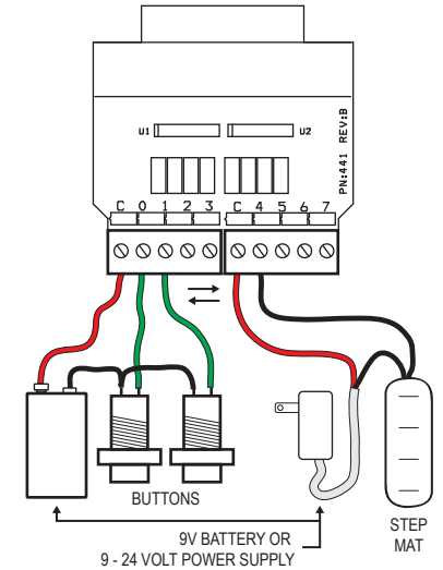
TRIGGERING FROM BUTTONS OR STEP MAT
