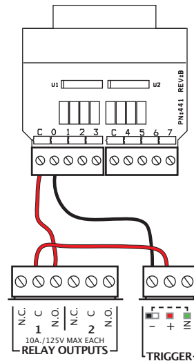
TRIGGERING FROM A RELAY OUTPUT (ALL PICOBOOS EXCEPT PICOBOO ONE)
