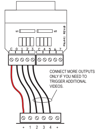
TRIGGERING FROM A SOLID-STATE OUTPUT (BOOBOX FLEX / FLEXMAX / PICOBOO ONE)
